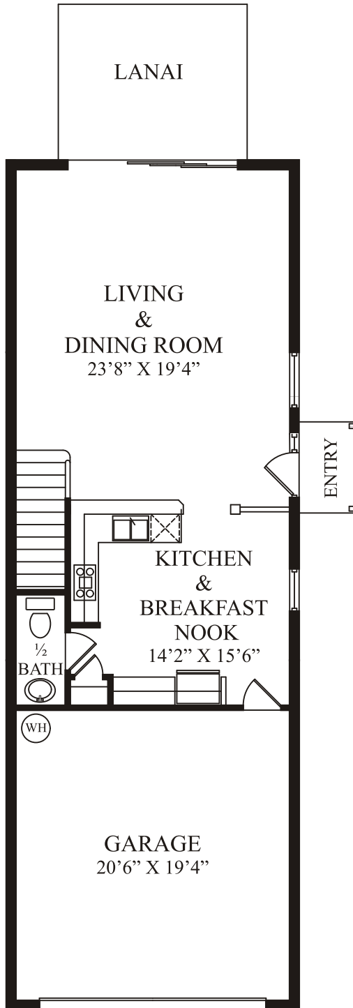
FIRST FLOOR
